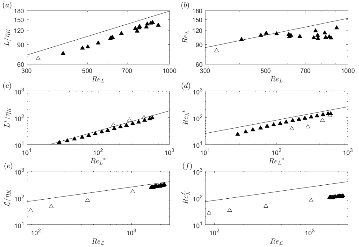
Figure 6.4: Dependence of (a) L/\eta_K and (b) Re_\lambda on Re_L , dependence of (c) L^*/\eta_K and (d) Re_\lambda^* on Re_L^* , and dependence of (e) \mathcal{L}/\eta_K and (f) Re_\lambda^{\mathcal{L}} on Re_{\mathcal{L}} . Symbols are as in Table (4.1). Solid symbols indicate measurement locations where y \leq 0.5\delta .
