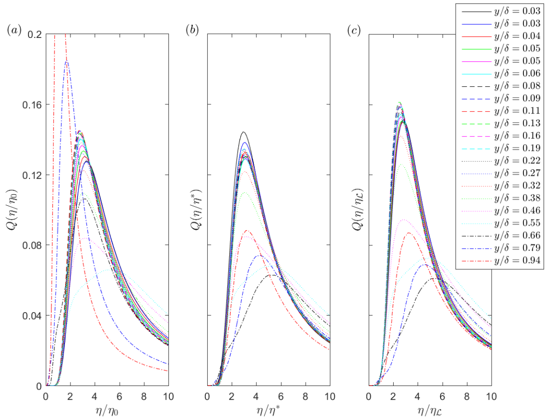
Figure B1: Measured PDFs of local dissipation scales for the case with a laminar free-stream condition using linear axes, normalized by: (a) \eta_0 ; (b) \eta^* ; and (c) \eta_{\mathcal{L}} from all measured positions within the boundary layer when the flow is intermittent.
