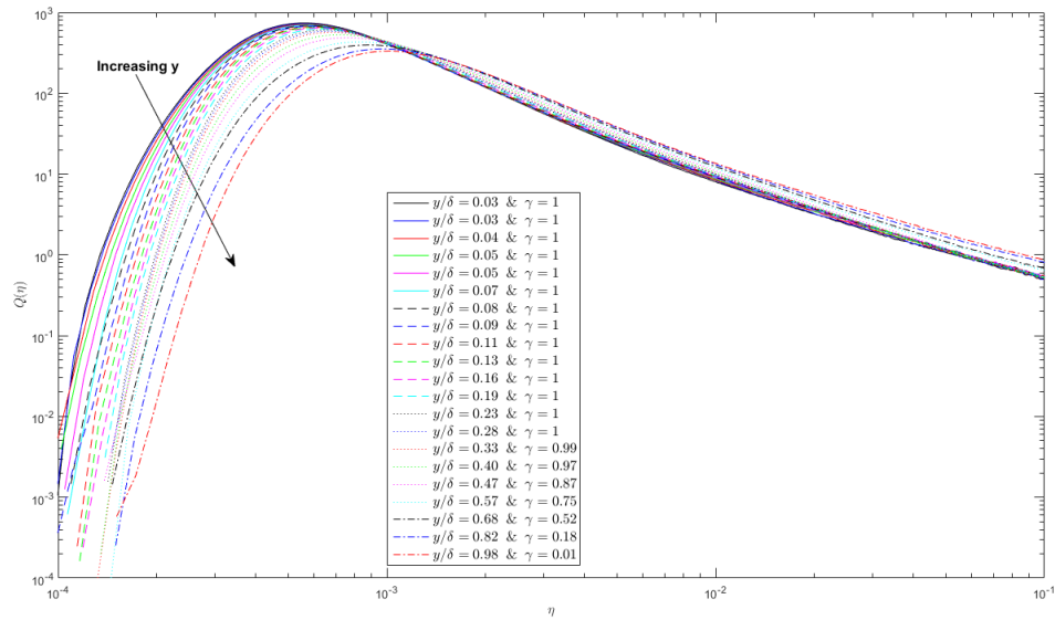
Figure 6.7: Forms of the PDFs of local dissipation scales from all measured positions within the boundary layer for the condition of a turbulent free-stream.
